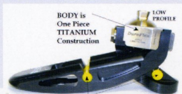
Interchangeable KEEL & HEEL Plugs for Custom Feel
